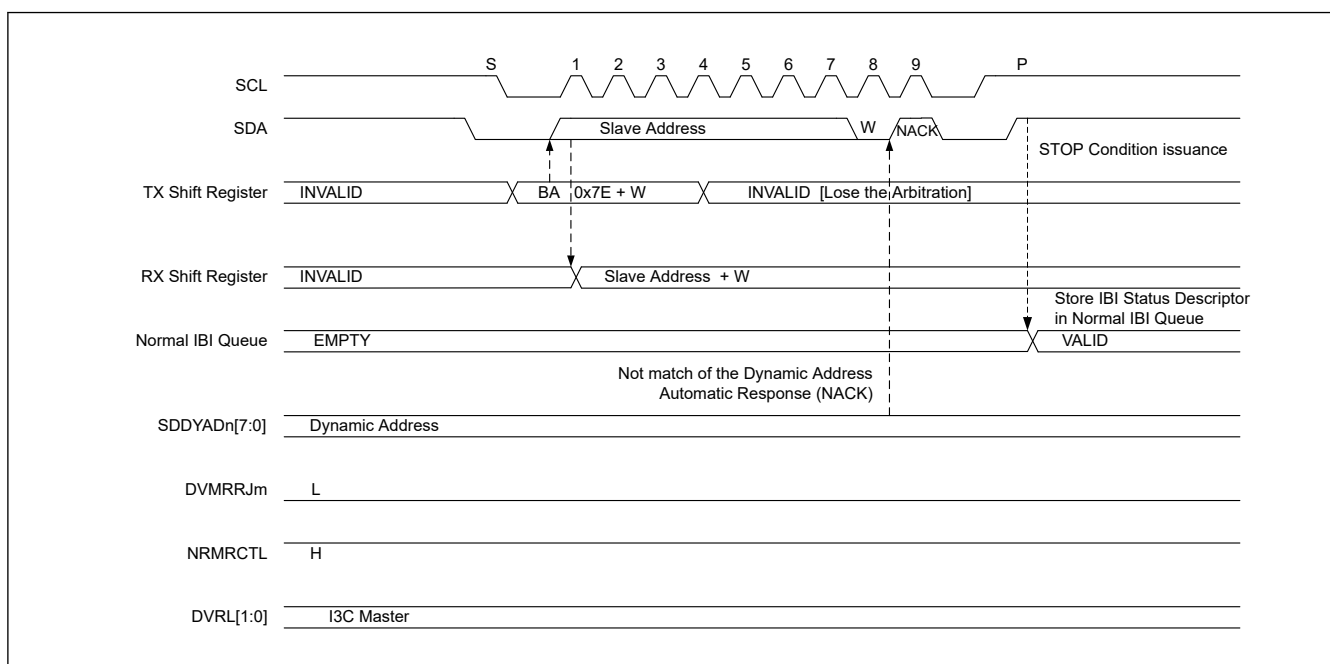
Figure 40.106 Mastership request : NACK (not match the DVDYAD[7:0] of DAT) and NRMCTL = 1
