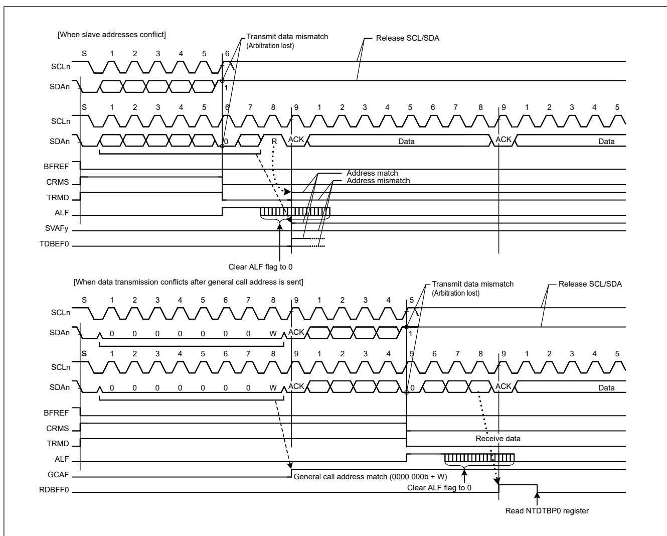
Figure 40.89 Examples of master arbitration-lost detection (MALE = 1)
