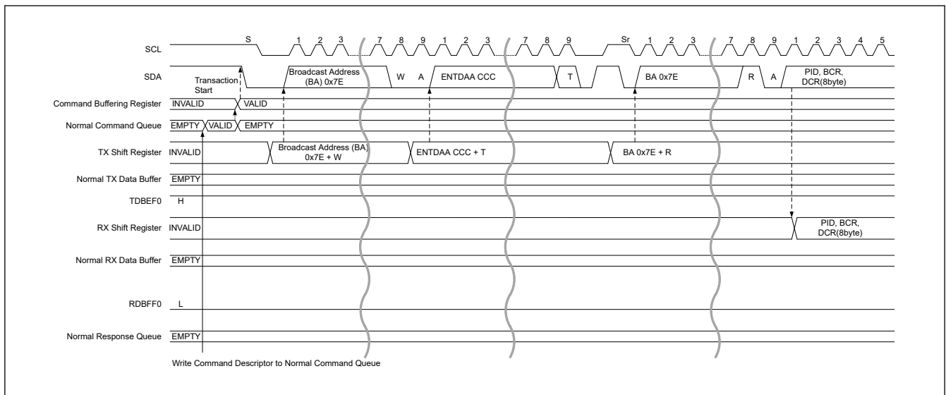
Figure 40.12 Dynamic address assign procedure (ENTDAA CCC) timing (1/3)
