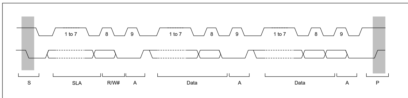
Figure 40.70 I 2 C bus timing (SLA = 7 bits)
