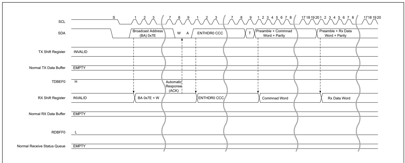
Figure 40.53 HDR data write transfer (HDR-DDR) timing (1/3)
