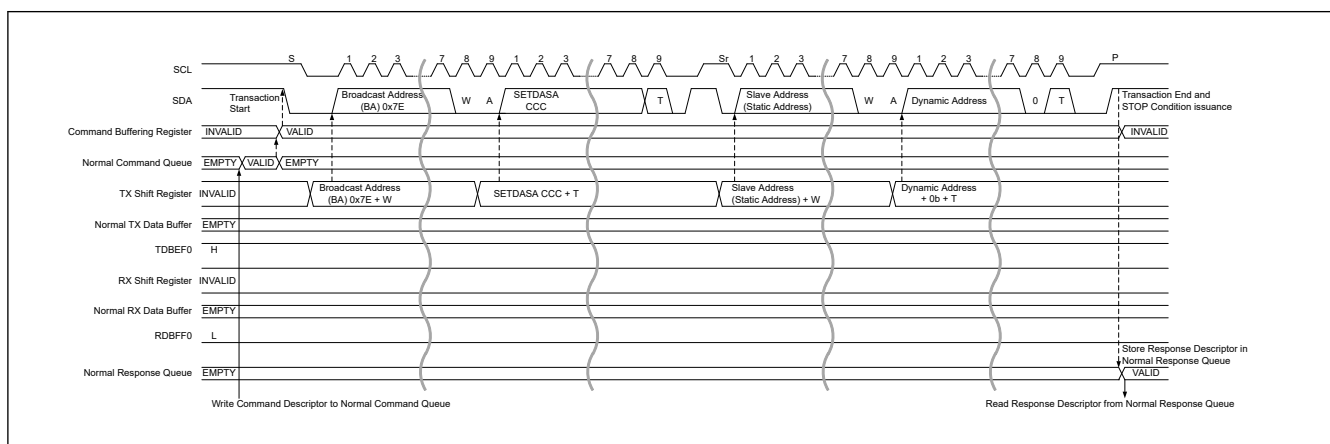
Figure 40.15 Dynamic address assign procedure (SETDASA CCC) timing
