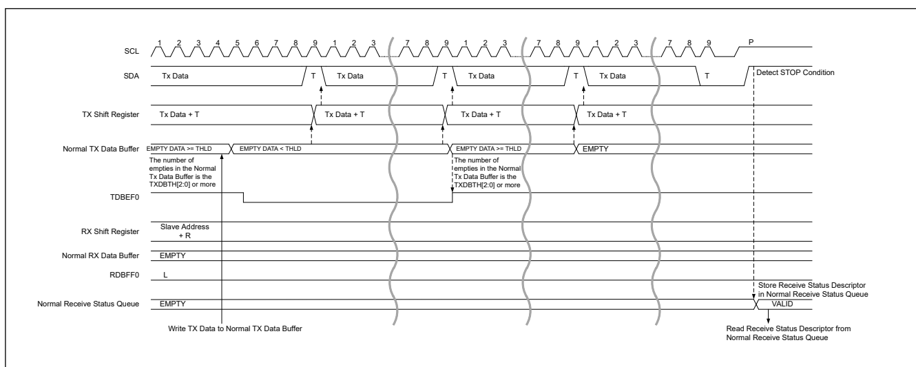
Figure 40.50 SDR data read transfer timing (2/2)
