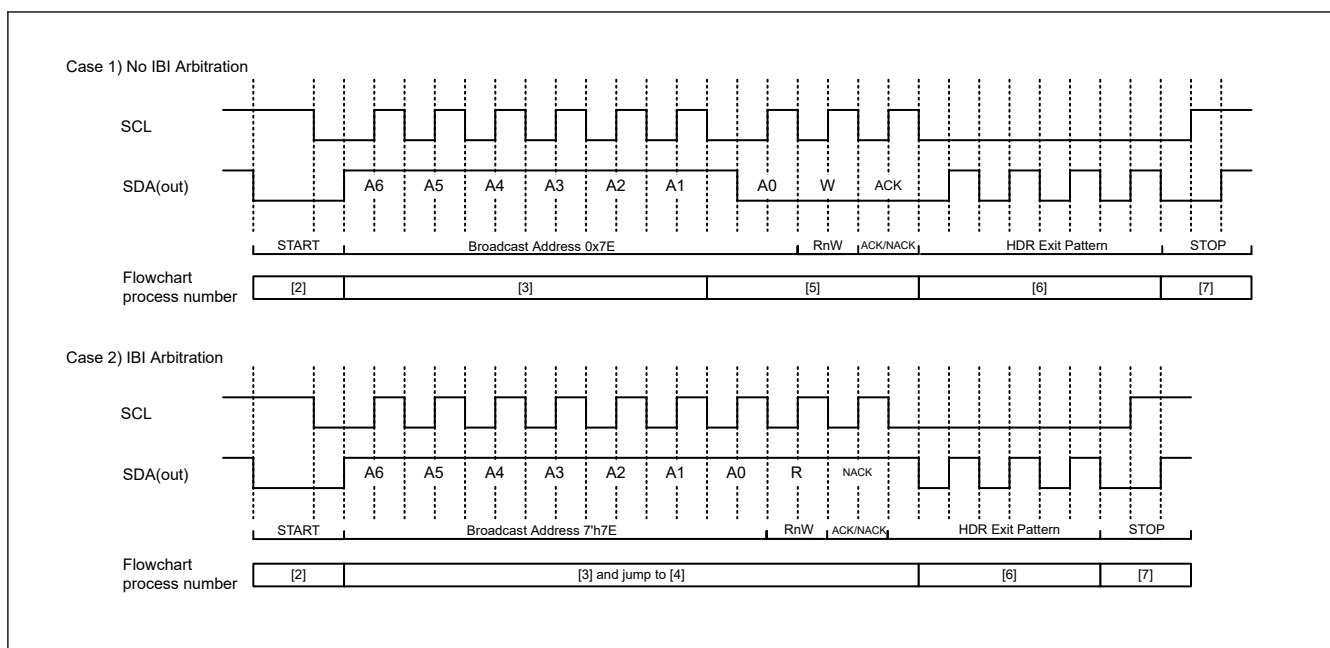
Figure 40.125 I3C Escalation Handling timing chart for I3C Master
