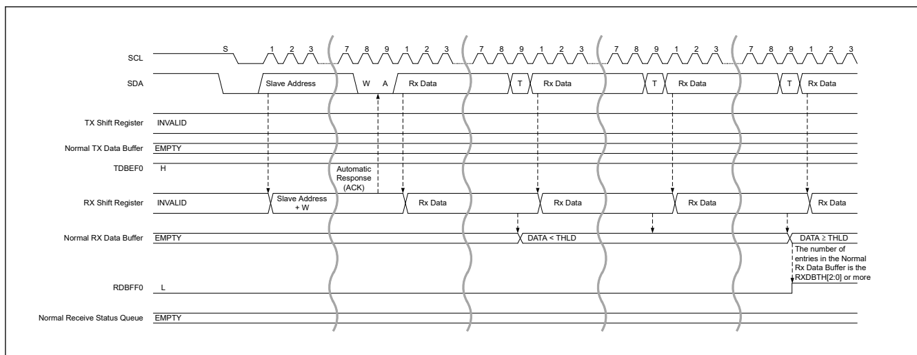
Figure 40.45 SDR data write transfer timing (1/2)
