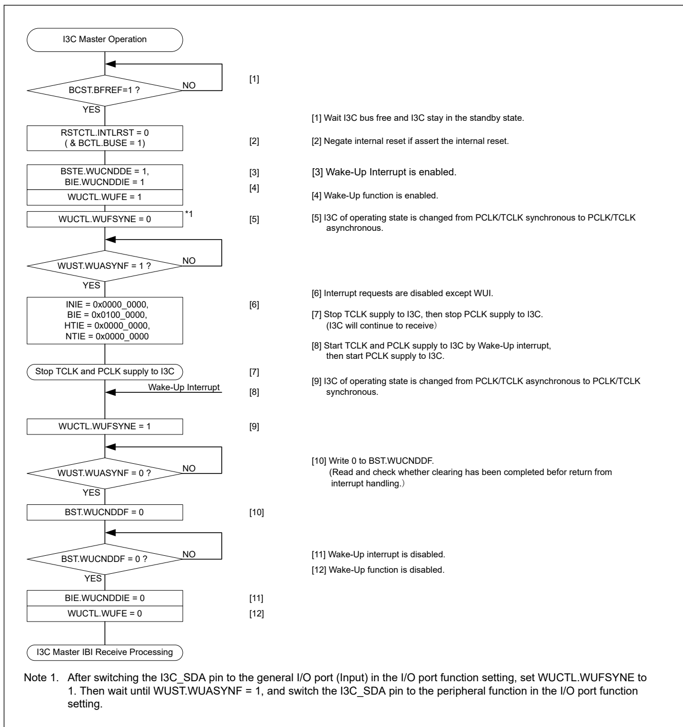
Figure 40.151 Use case of I3C master wake-up
