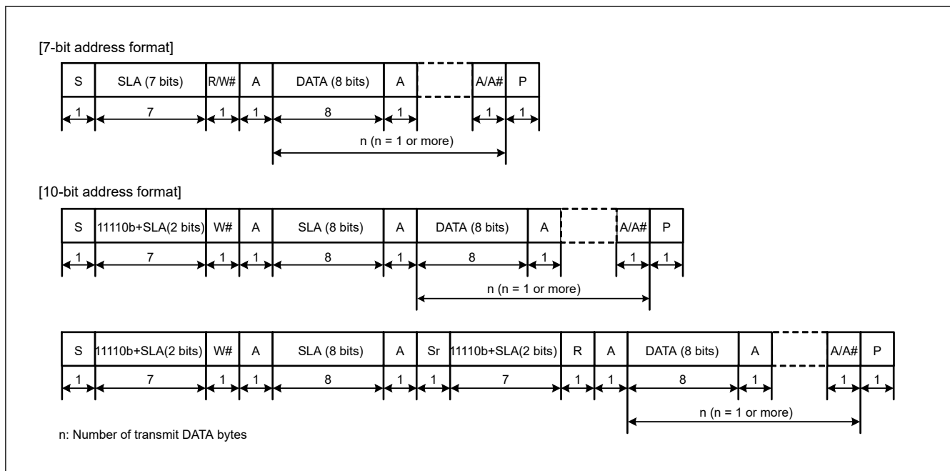
Figure 40.69 I 2 C bus format
