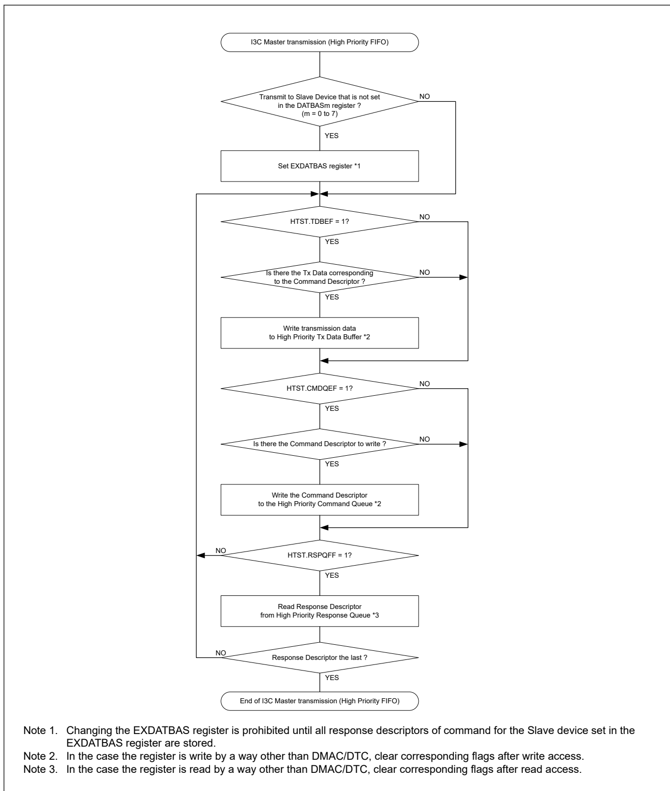
Figure 40.148 Example of I3C master transmission flowchart (high priority FIFO buffer transfer)
